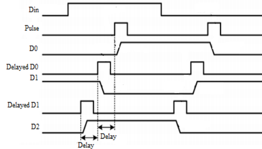
Figure 4.b Output of the LFSR with delayed pulse circuit
