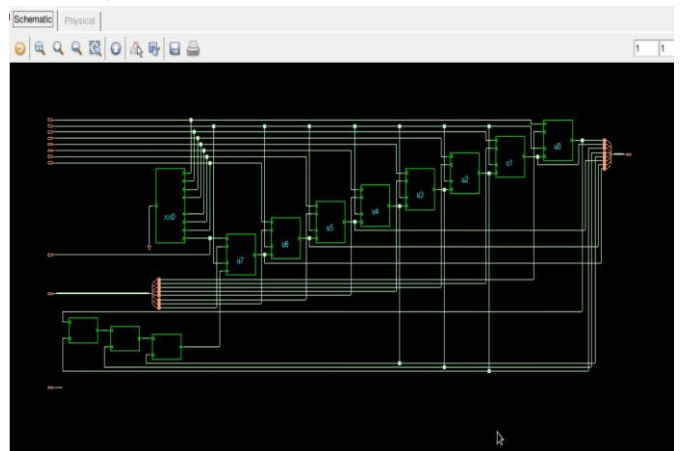
Figure 8 RTL schematic of proposed LFSR
