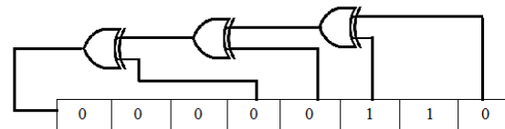
Figure 1. 8-bit LFSR circuit
