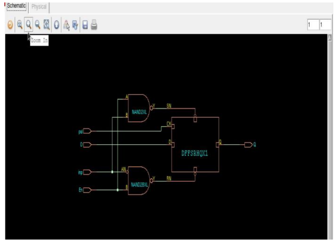
Figure 7 RTL schematic of D latch
