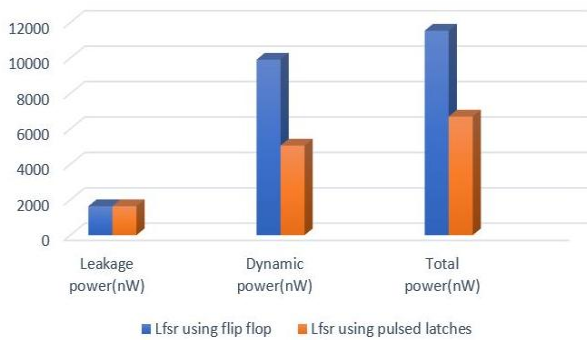
Figure 6. Power comparison chart
