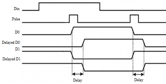
Figure 5.b Output of the LFSR with delayed circuit
