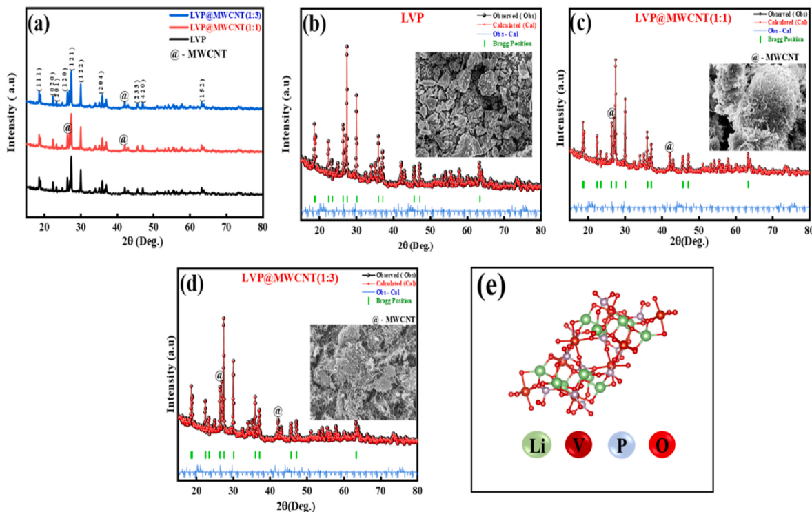
Fig. 2. (a) Diffraction pattern of the pure LVP and carbon coated LVP samples; Rietveld refinement of (b) pristine LVP (c) LVP@MWCNT (1:1); (d) LVP@MWCNT (1:3); (e) refined structure of LVP.
