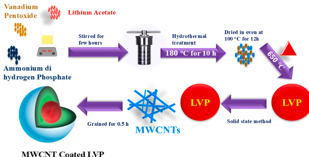
Fig. 1. A simplified representation of the steps used to create LVP coated with MWCNTs.
